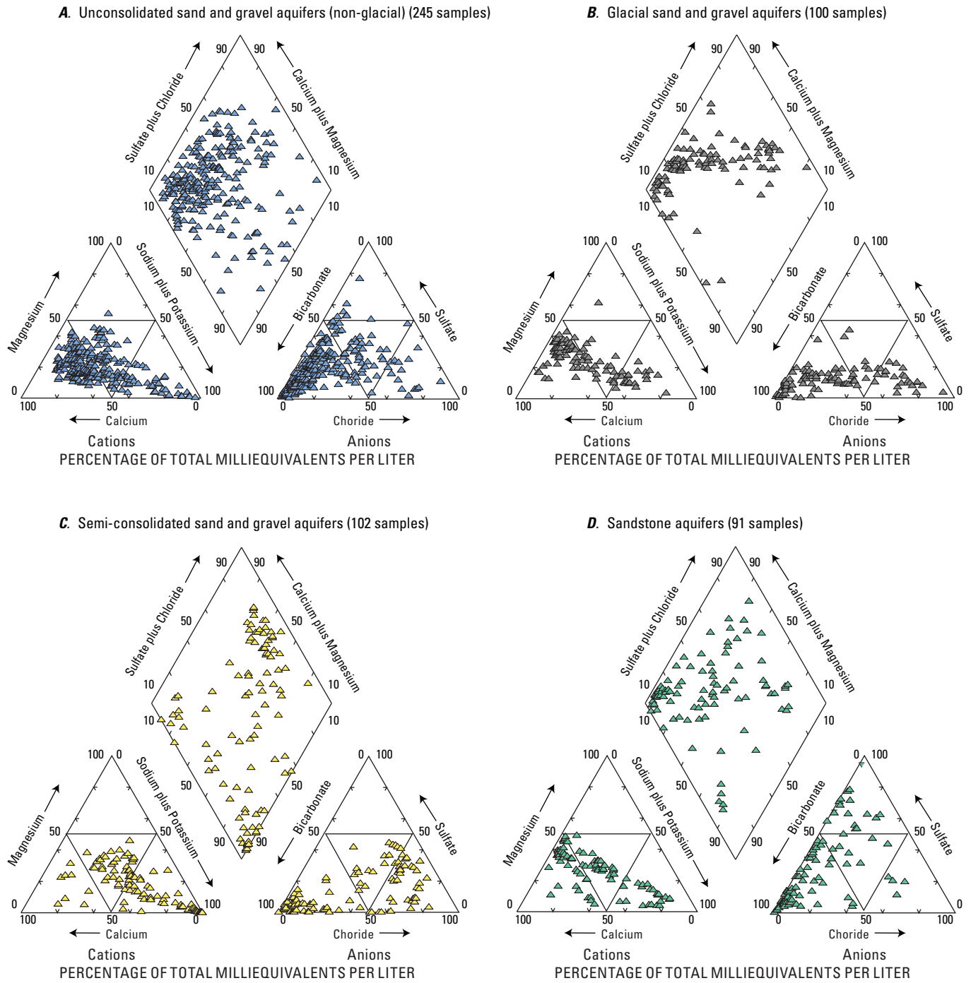
Figure 17. Ionic composition of source water from public-well samples collected during 1993–2007, by principal aquifer rock type. Data are from 733 samples in which all required cations (calcium, magnesium, sodium, potassium) and anions (chloride, bicarbonate, and sulfate) were analyzed.
